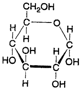
Glucose
